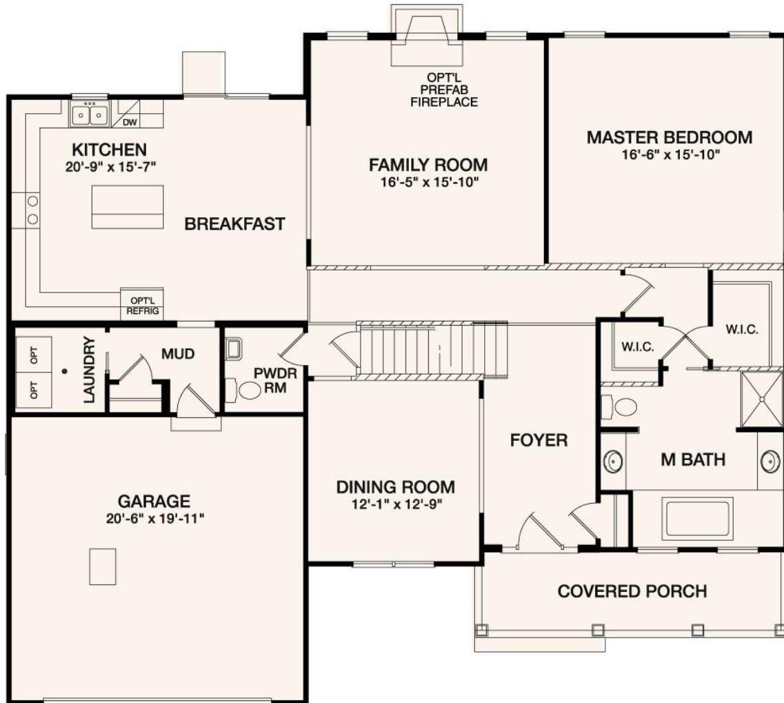
First Floor
