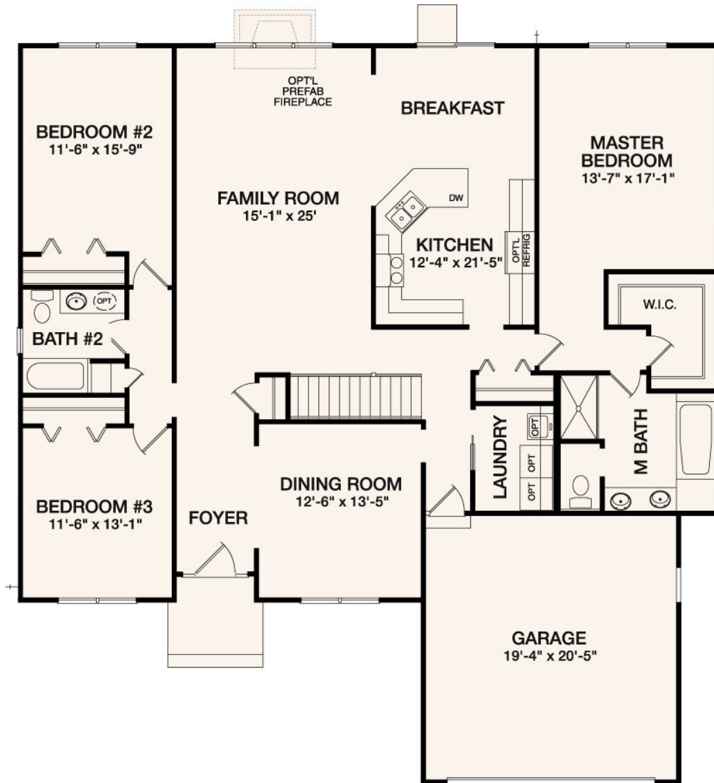
First Floor
